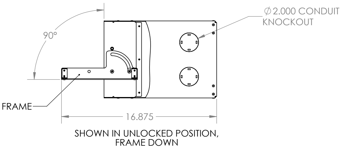
VIEW A-A SCALE 1 : 6
