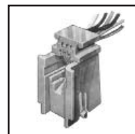
70-505 (623D4) Modular line cord female chassis jack. 6-position, 4 wires and lugs. For use in phone base.
